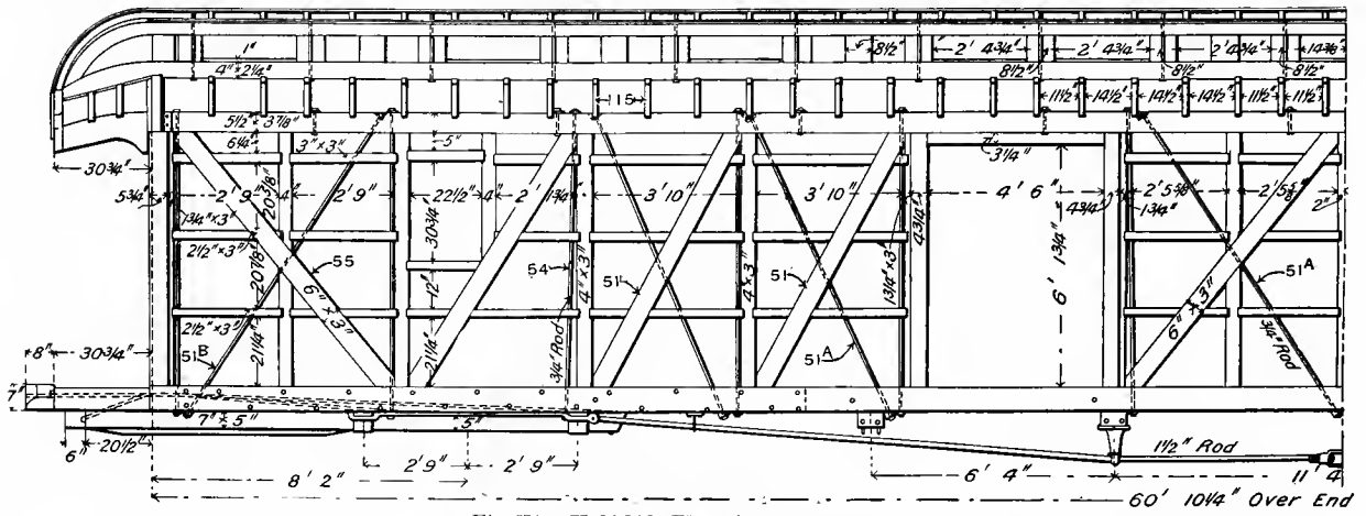
Fig. 574. Half Side Elevation of Framing.
